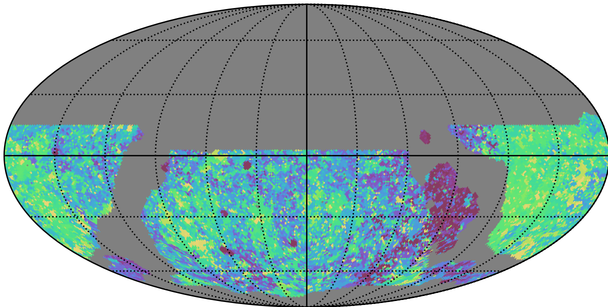
noroll_mjdp365_v3.4_10yrs WFD g band: Max Inter-Night Gap
