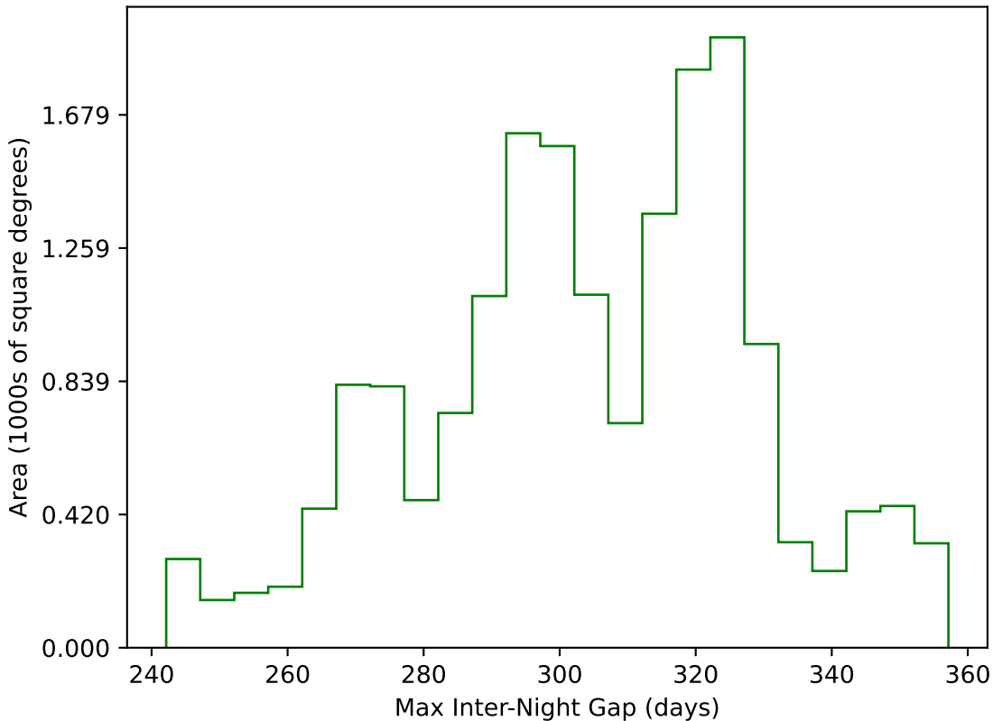
noroll_mjdp365_v3.4_10yrs WFD g band: Max Inter-Night Gap
