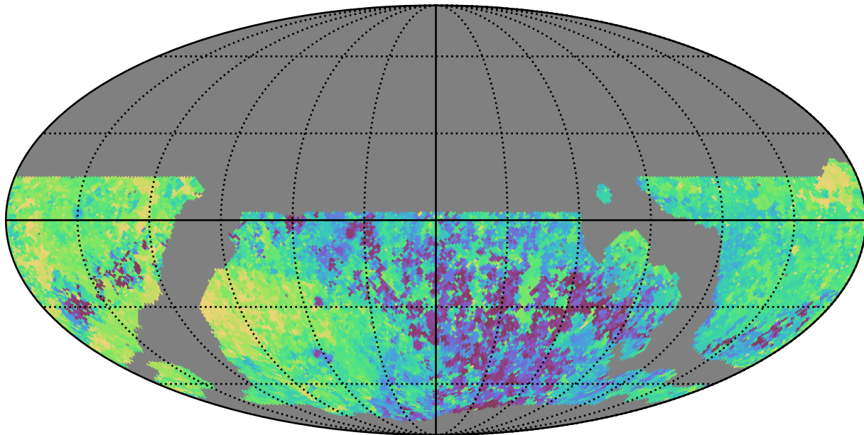
noroll_mjdp365_v3.4_10yrs WFD all bands: Max Inter-Night Gap
