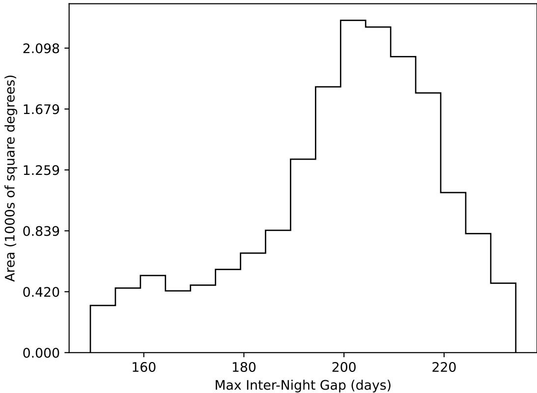
noroll_mjdp365_v3.4_10yrs WFD all bands: Max Inter-Night Gap
