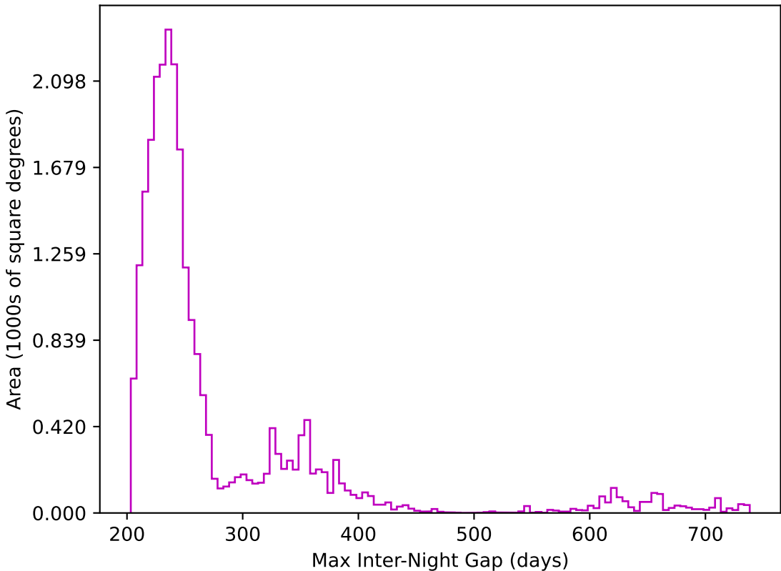
noroll_mjdp365_v3.4_10yrs All sky z band: Max Inter-Night Gap
