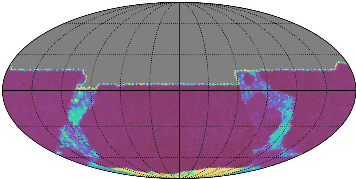
noroll_mjdp365_v3.4_10yrs All sky y band: Max Inter-Night Gap
