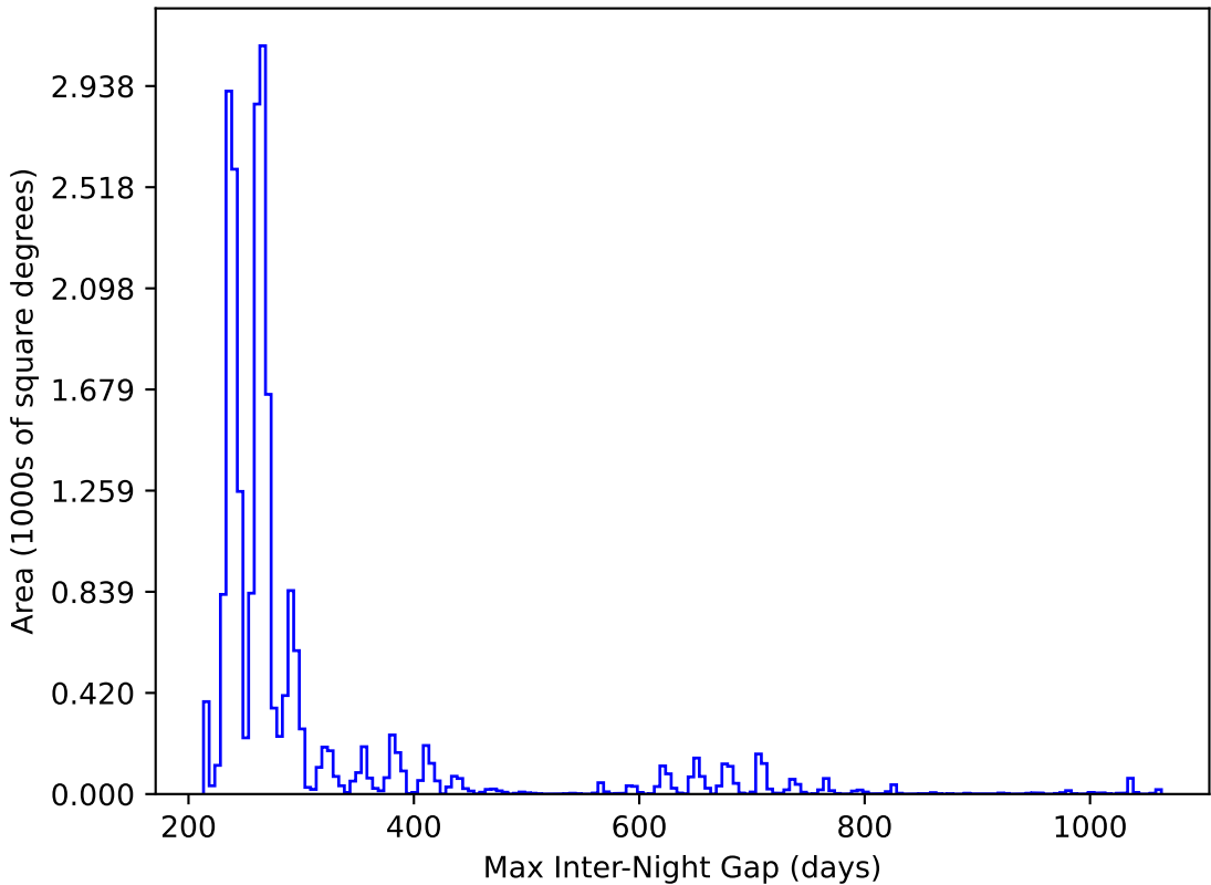
noroll_mjdp365_v3.4_10yrs All sky y band: Max Inter-Night Gap
