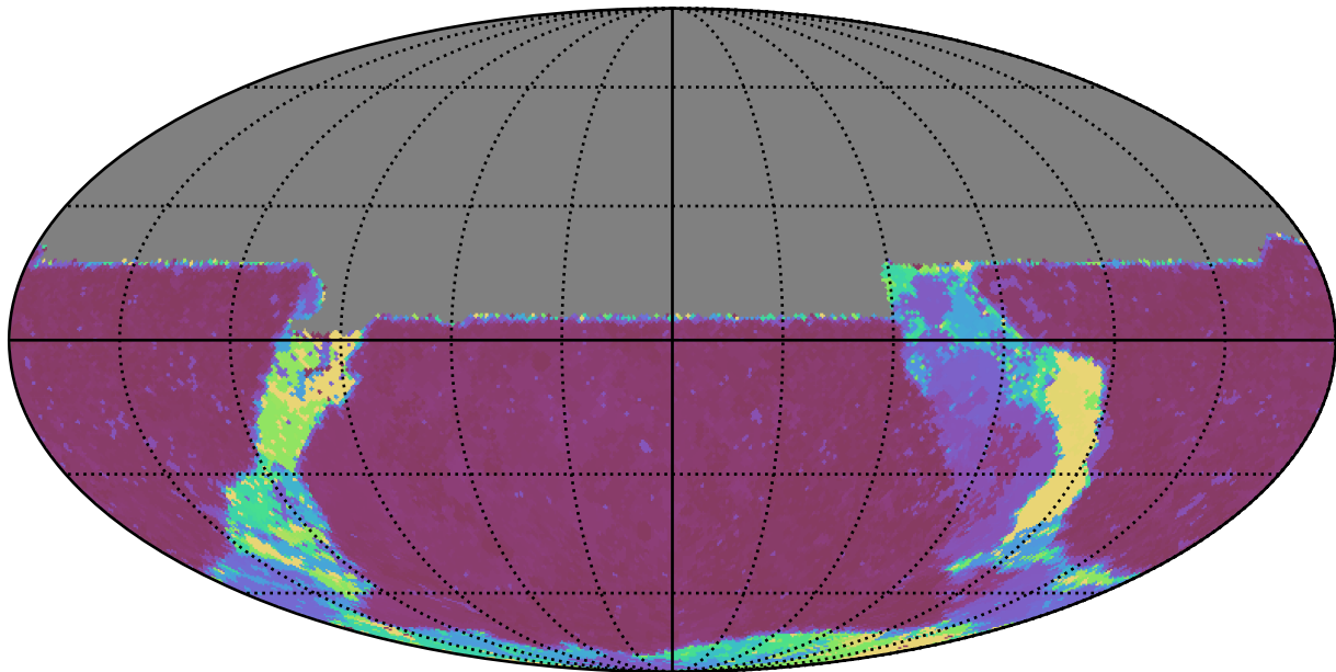
noroll_mjdp365_v3.4_10yrs All sky u band: Max Inter-Night Gap
