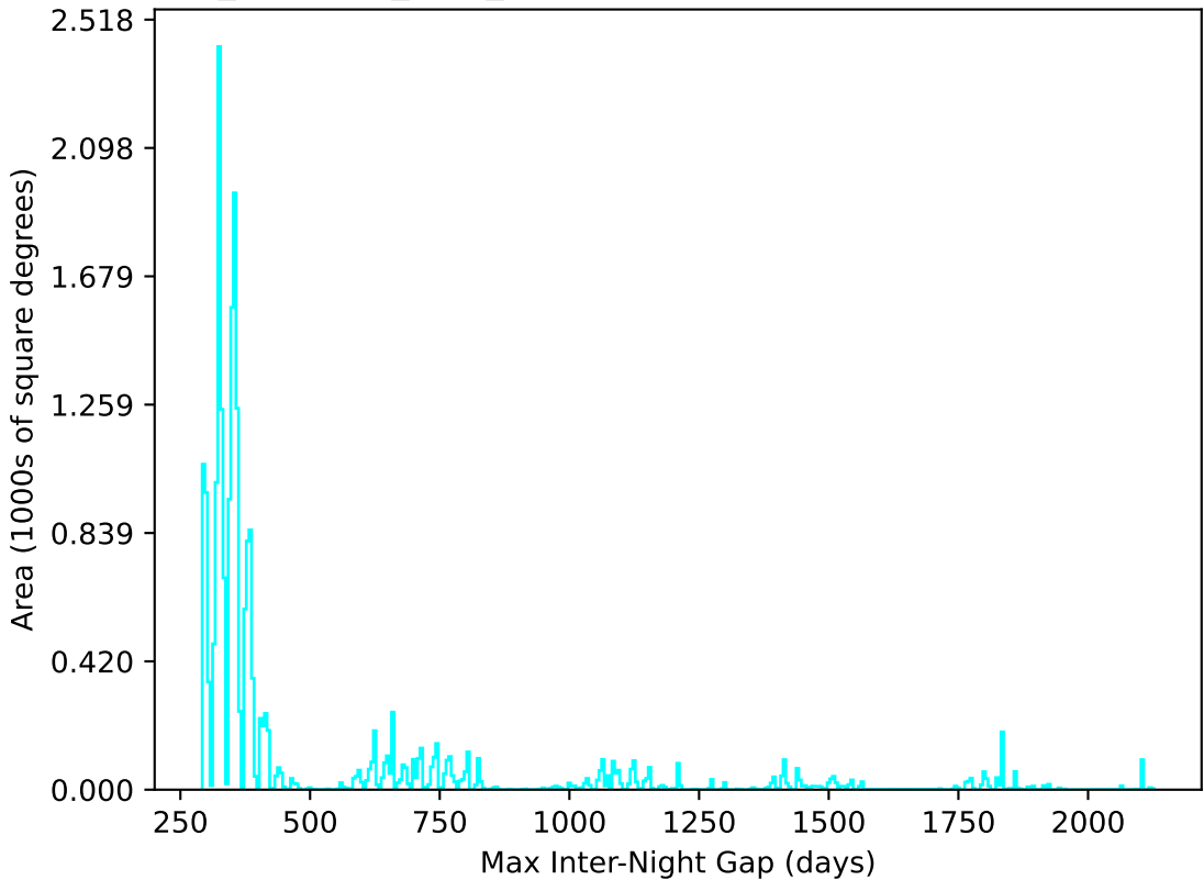
noroll_mjdp365_v3.4_10yrs All sky u band: Max Inter-Night Gap
