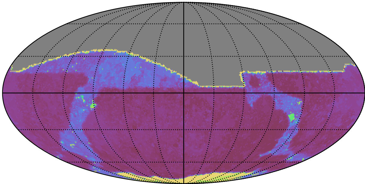
noroll_mjdp365_v3.4_10yrs All sky r band: Max Inter-Night Gap
