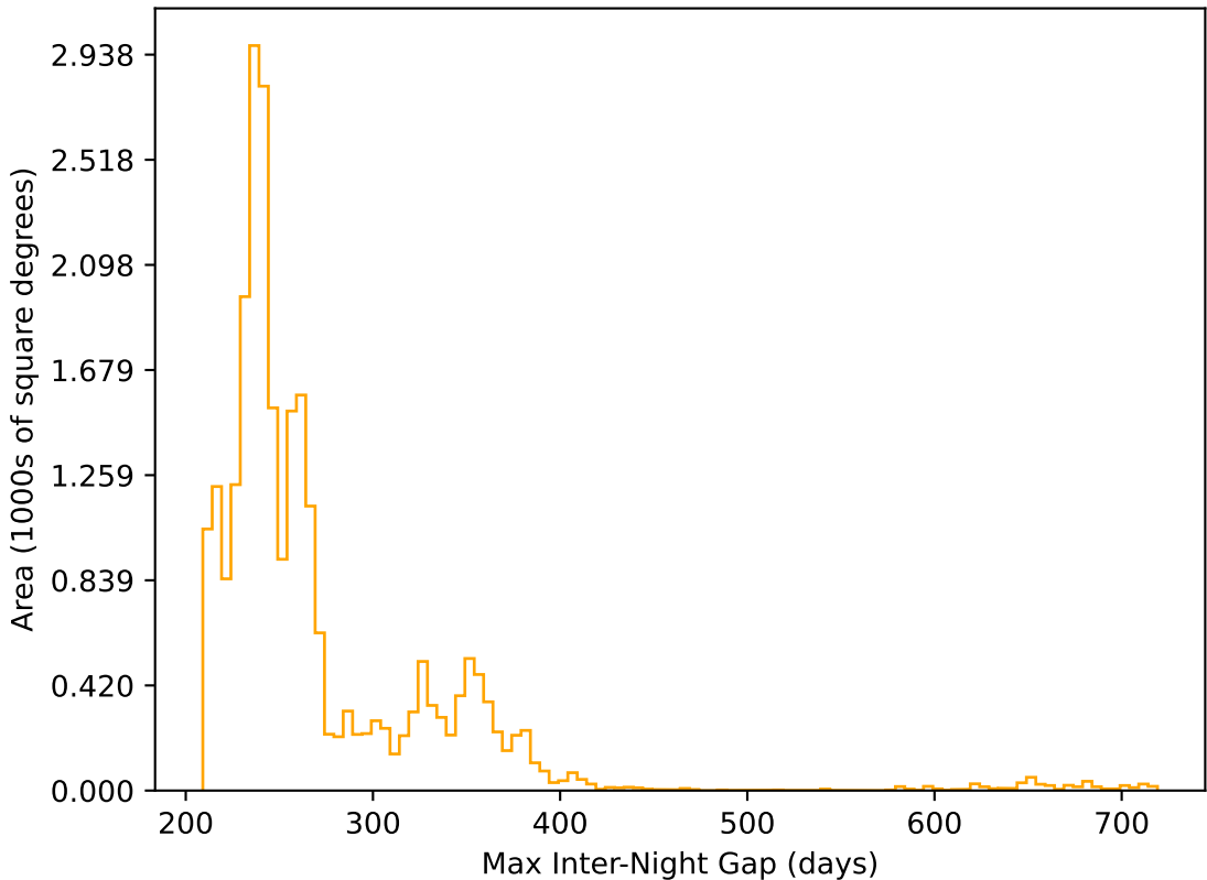
noroll_mjdp365_v3.4_10yrs All sky r band: Max Inter-Night Gap
