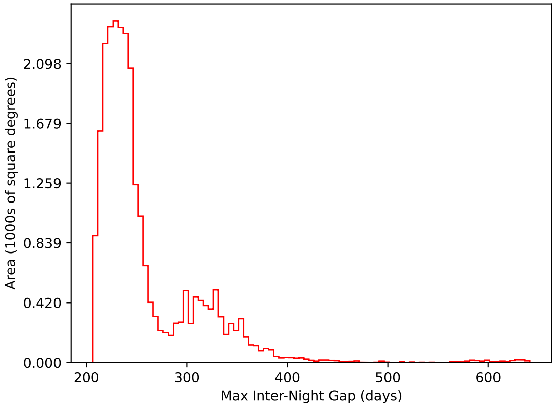
noroll_mjdp365_v3.4_10yrs All sky i band: Max Inter-Night Gap
