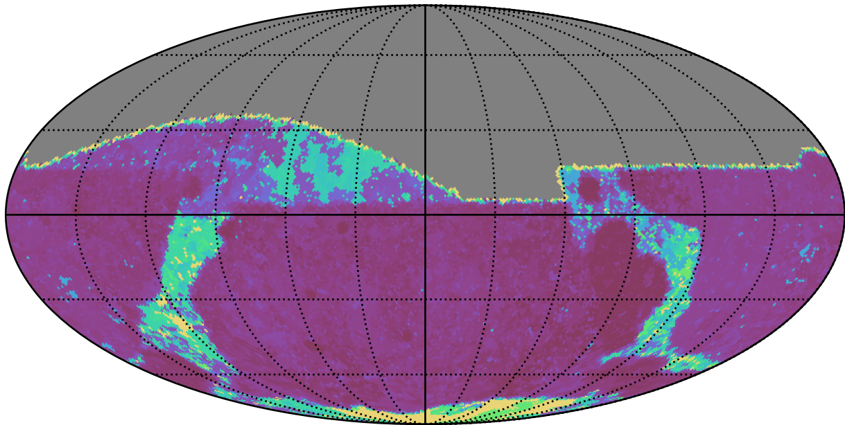
noroll_mjdp365_v3.4_10yrs All sky g band: Max Inter-Night Gap
