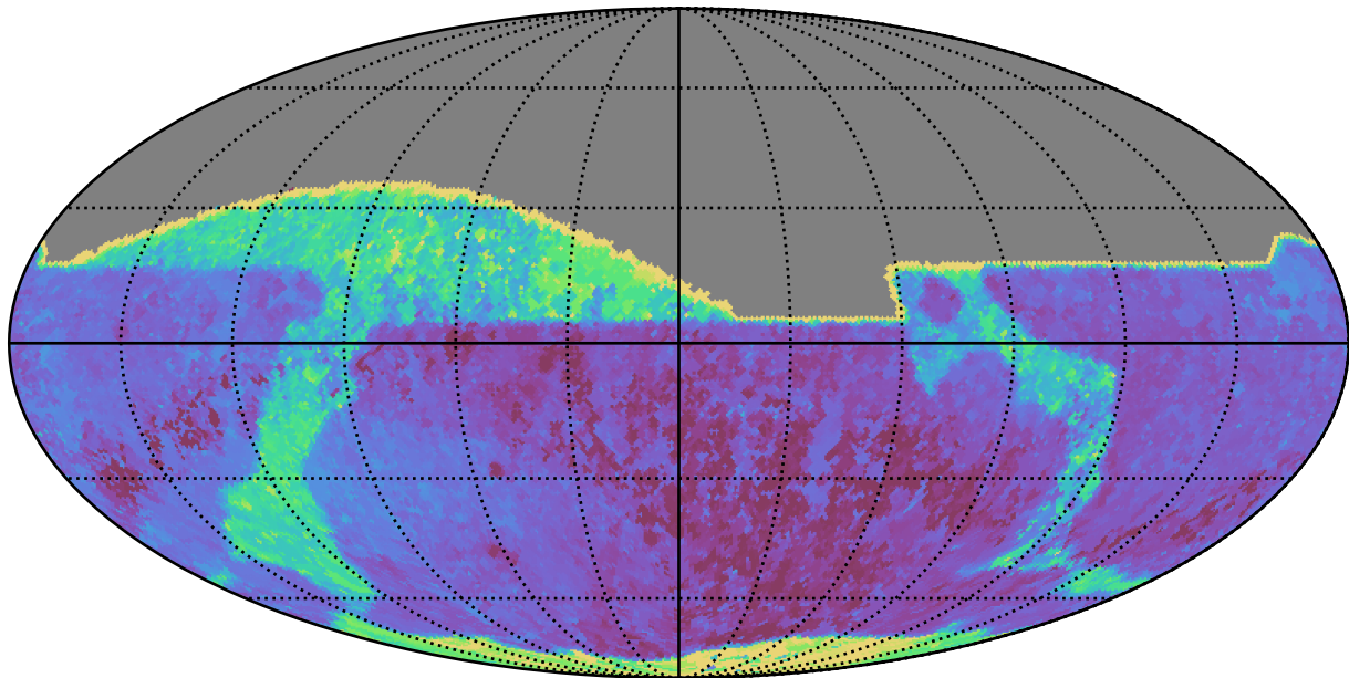
noroll_mjdp365_v3.4_10yrs All sky all bands: Max Inter-Night Gap
