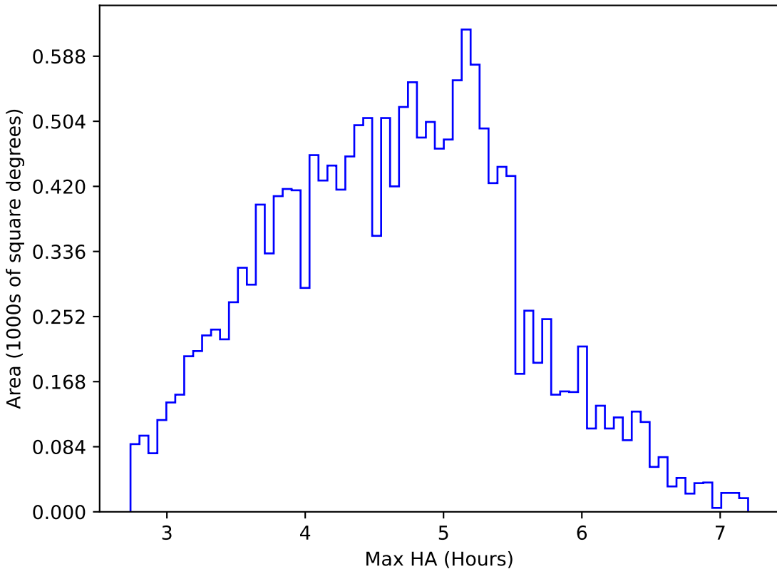
noroll_mjdp365_v3.4_10yrs WFD z band: Max HA
