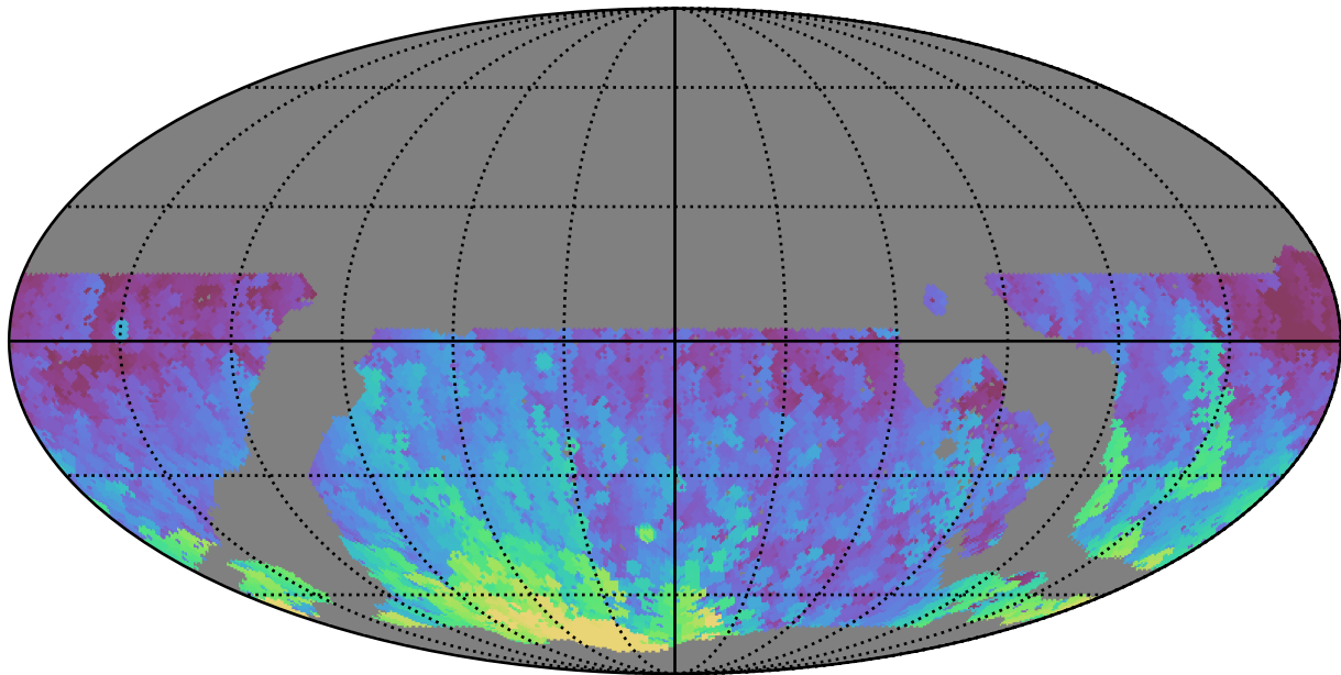
noroll_mjdp365_v3.4_10yrs WFD u band: Max HA
