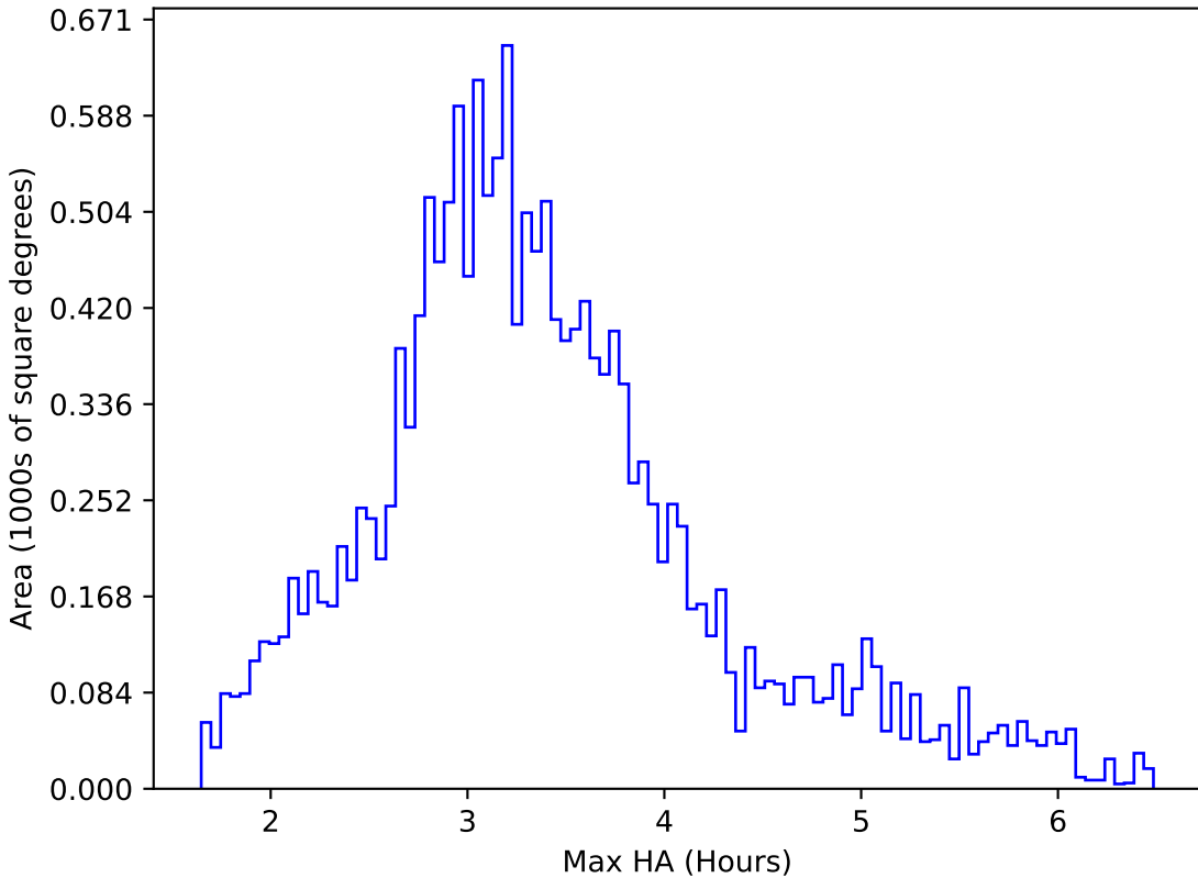
noroll_mjdp365_v3.4_10yrs WFD u band: Max HA
