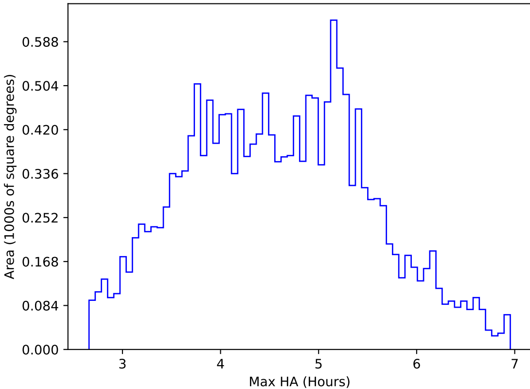
noroll_mjdp365_v3.4_10yrs WFD i band: Max HA
