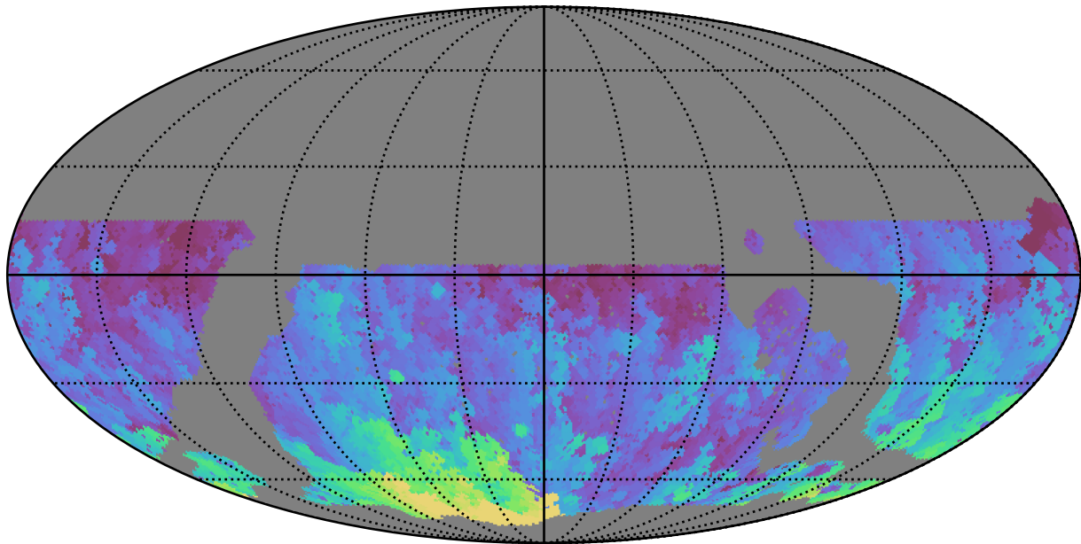
noroll_mjdp365_v3.4_10yrs WFD g band: Max HA
