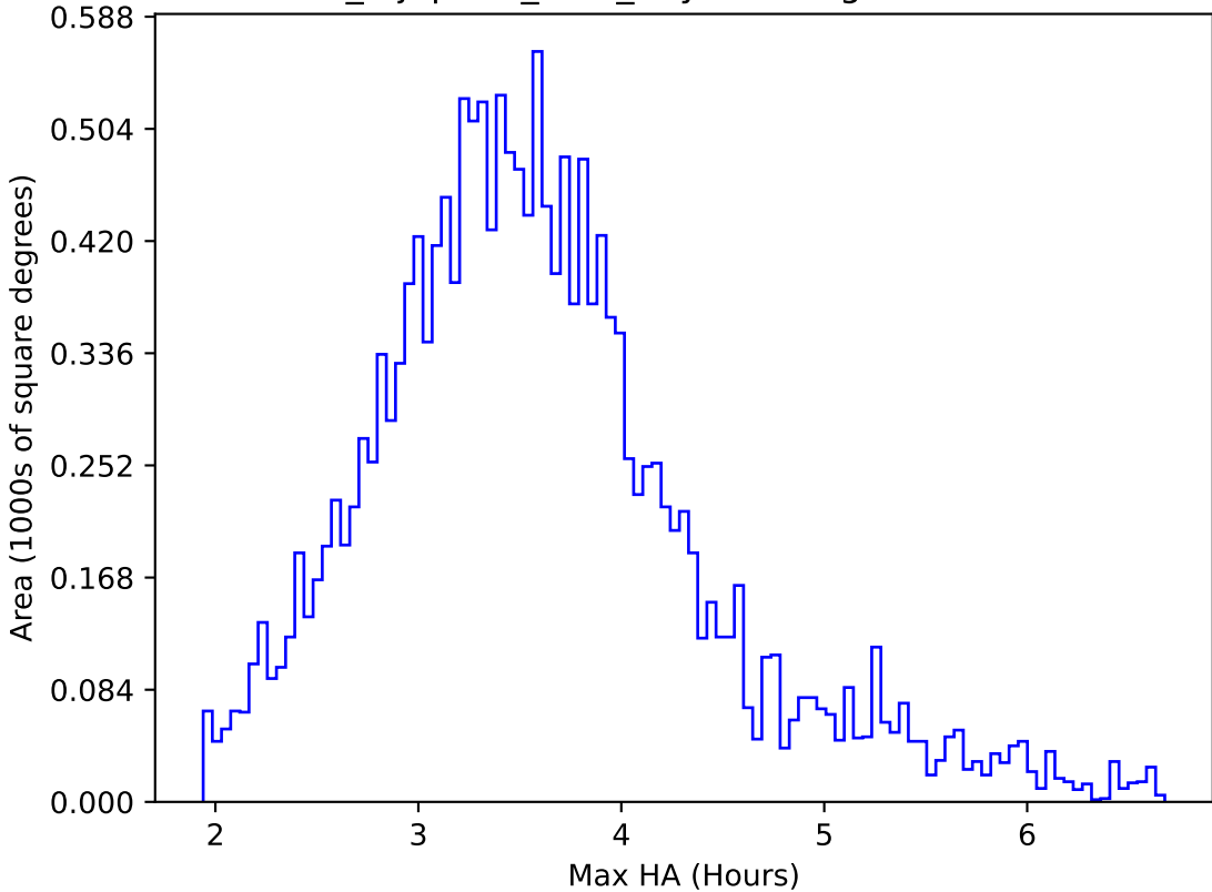
noroll_mjdp365_v3.4_10yrs WFD g band: Max HA
