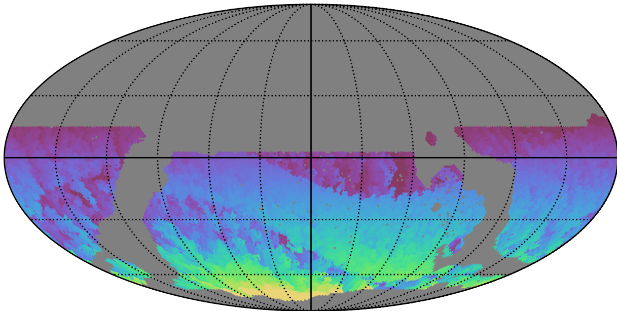
noroll_mjdp365_v3.4_10yrs WFD all bands: Max HA
