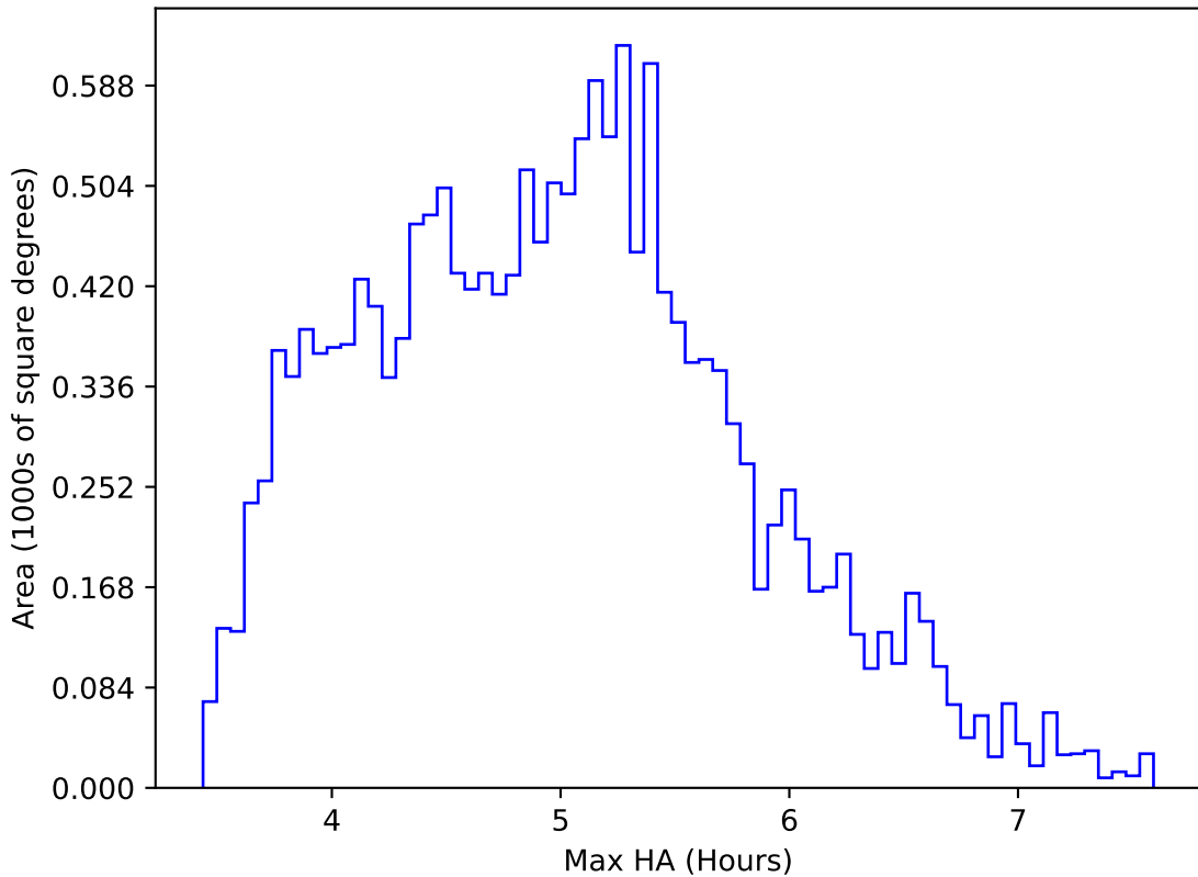
noroll_mjdp365_v3.4_10yrs WFD all bands: Max HA
