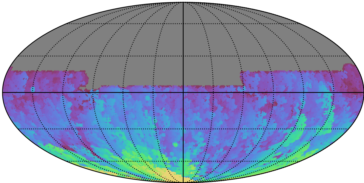
noroll_mjdp365_v3.4_10yrs All sky u band: Max HA
