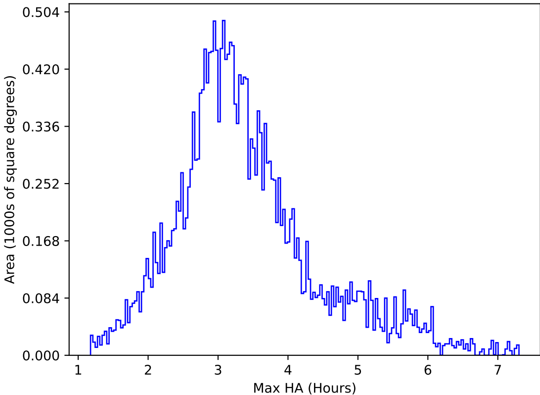
noroll_mjdp365_v3.4_10yrs All sky u band: Max HA
