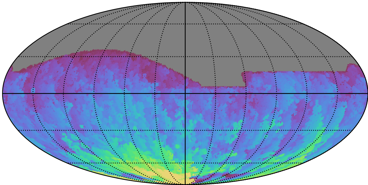
noroll_mjdp365_v3.4_10yrs All sky r band: Max HA
