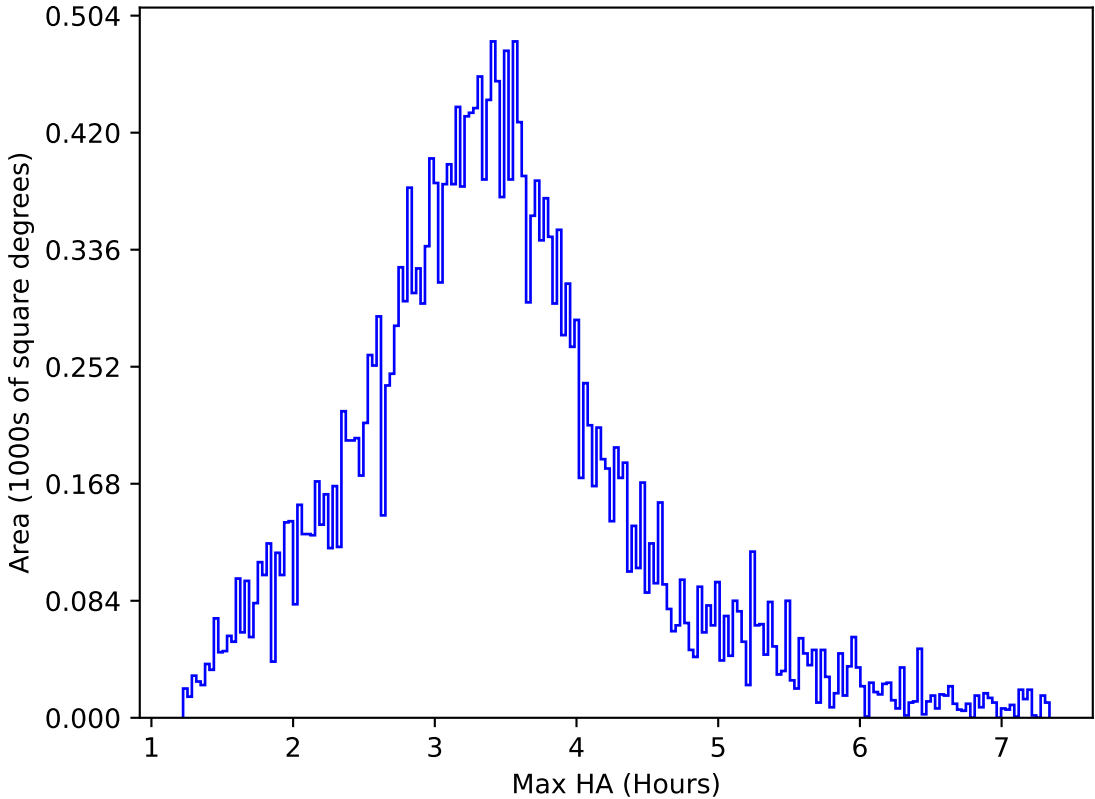
noroll_mjdp365_v3.4_10yrs All sky g band: Max HA
