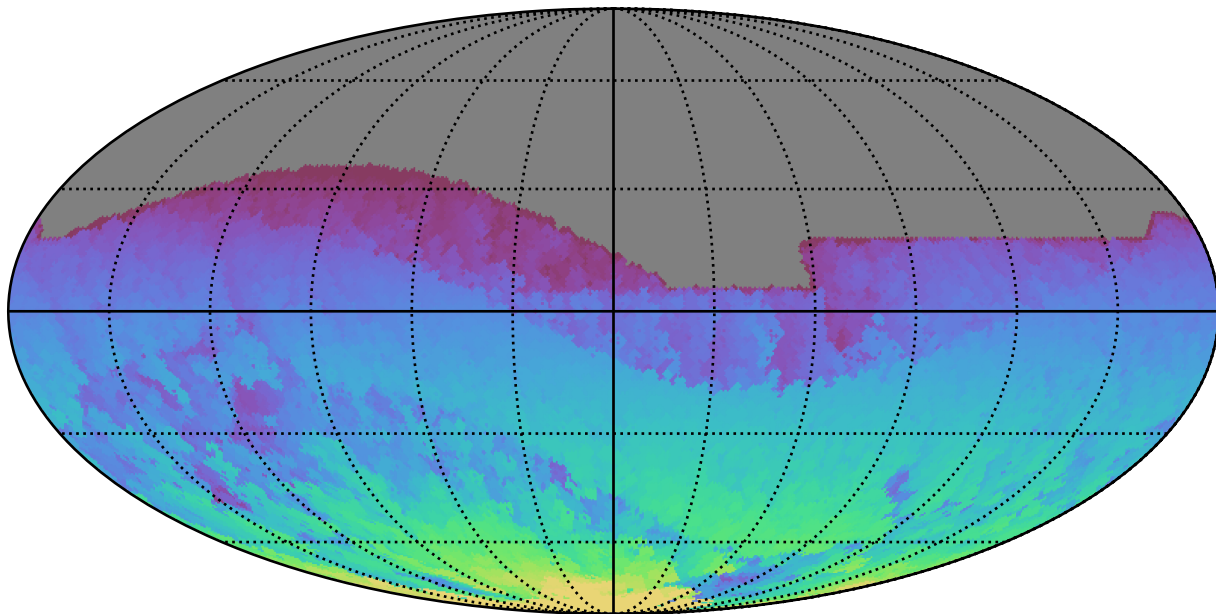
noroll_mjdp365_v3.4_10yrs All sky all bands: Max HA
