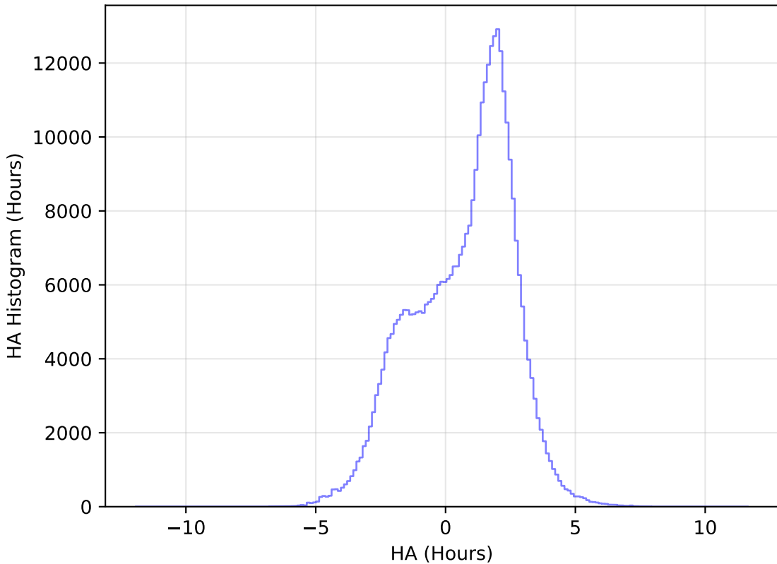
noroll_mjdp365_v3.4_10yrs WFD y band: HA Histogram
