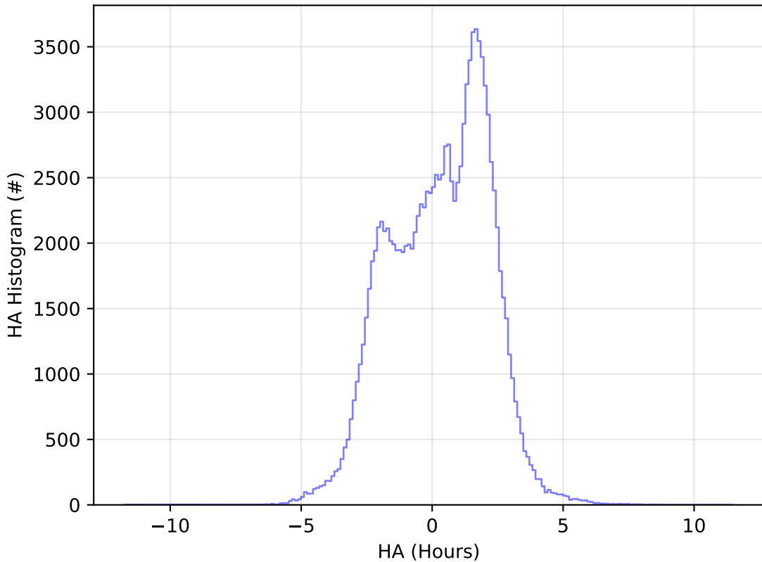
noroll_mjdp365_v3.4_10yrs WFD u band: HA Histogram
