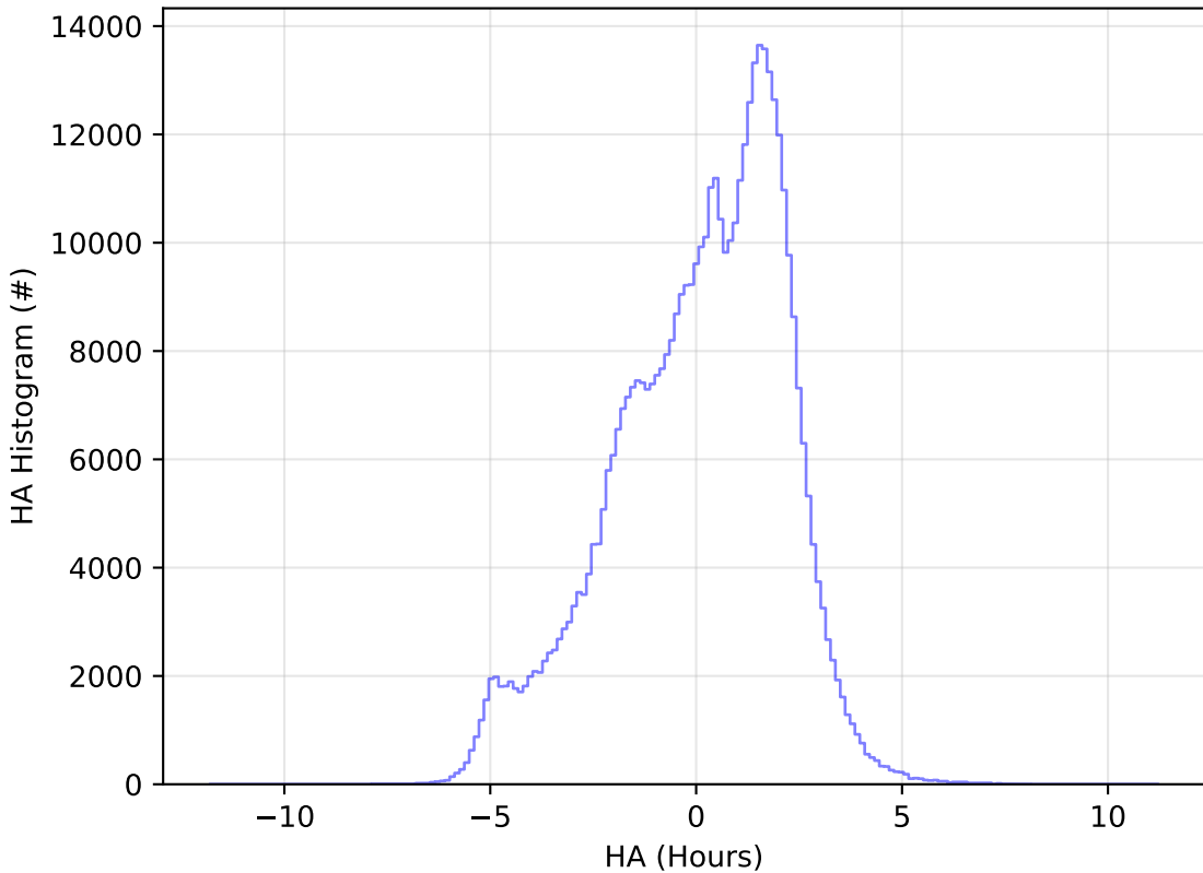
noroll_mjdp365_v3.4_10yrs WFD r band: HA Histogram
