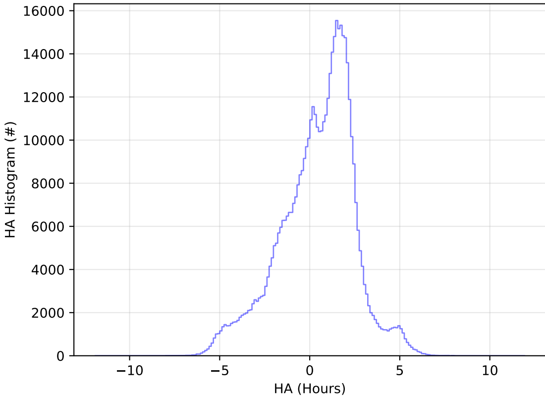
noroll_mjdp365_v3.4_10yrs WFD i band: HA Histogram
