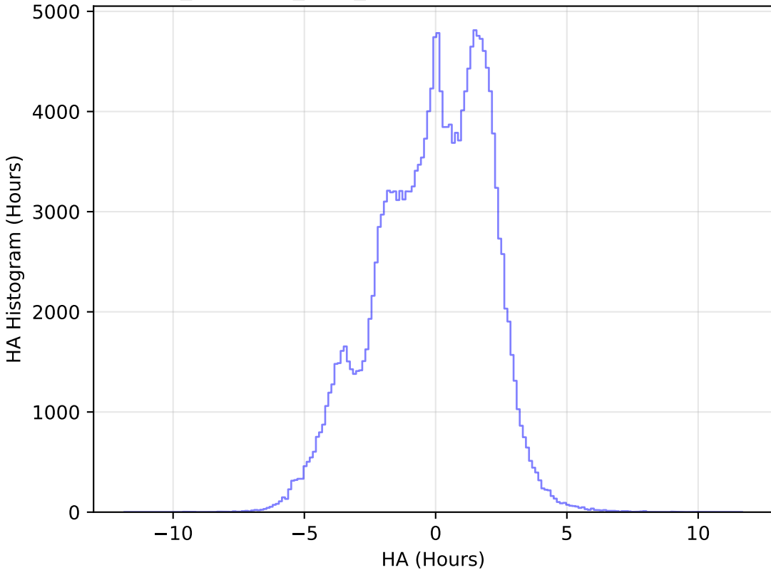
noroll_mjdp365_v3.4_10yrs WFD g band: HA Histogram
