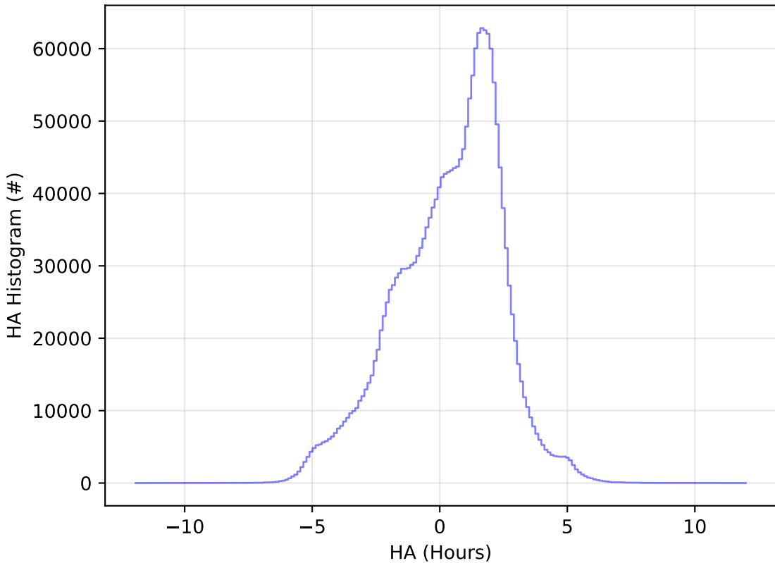
noroll_mjdp365_v3.4_10yrs WFD all bands: HA Histogram
