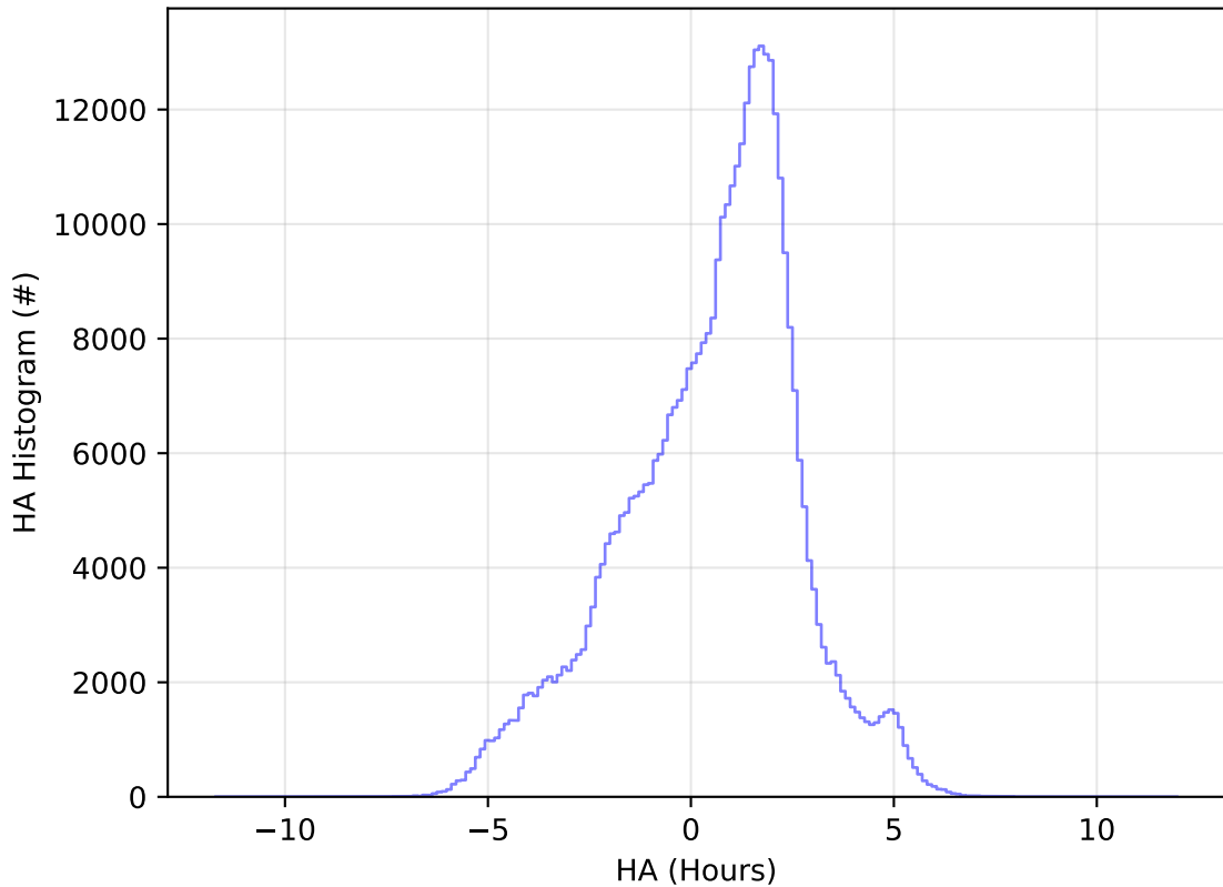
noroll_mjdp365_v3.4_10yrs All sky z band: HA Histogram
