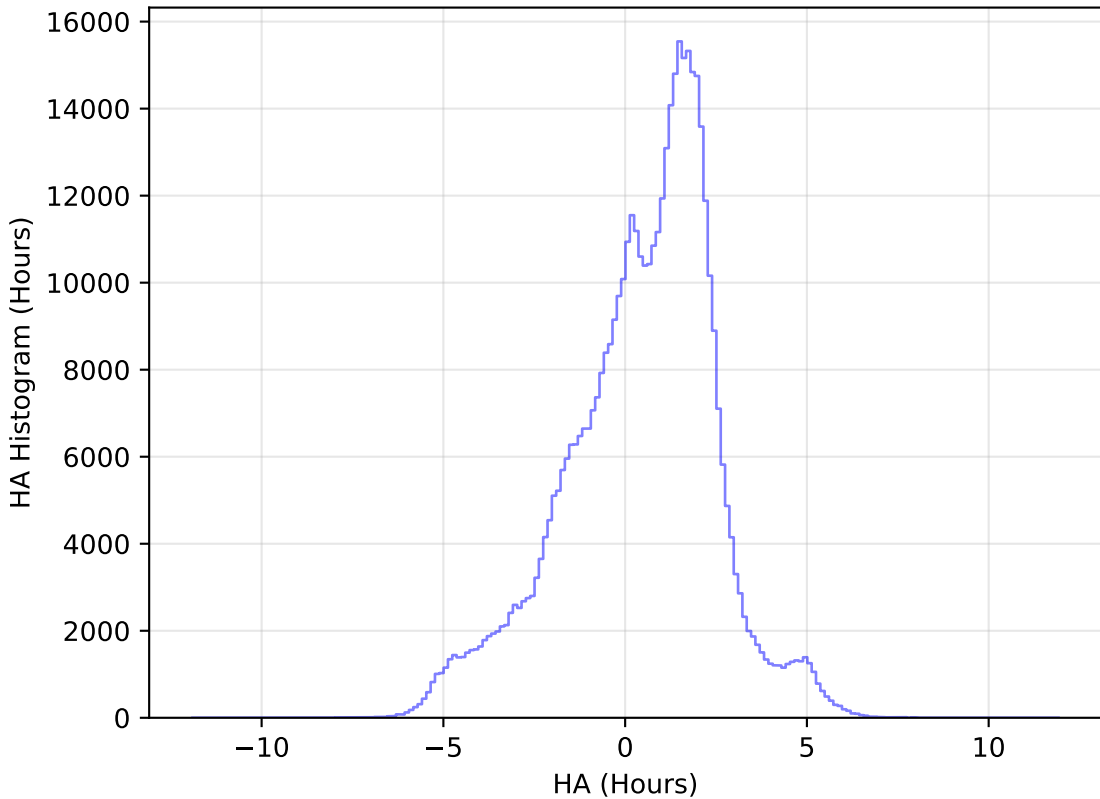
noroll_mjdp365_v3.4_10yrs All sky i band: HA Histogram
