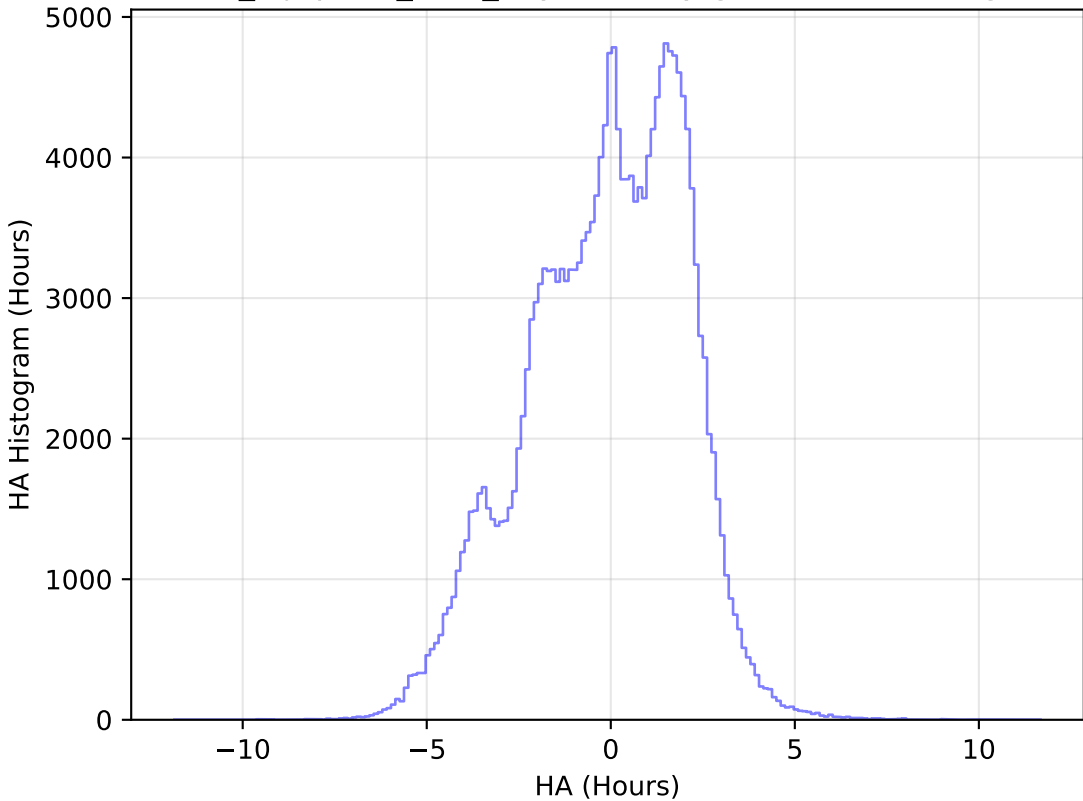
noroll_mjdp365_v3.4_10yrs All sky g band: HA Histogram
