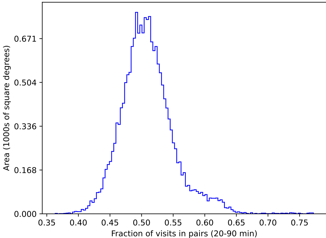
noroll_mjdp365_v3.4_10yrs gri WFD: Fraction of visits in pairs (20-90 min)
