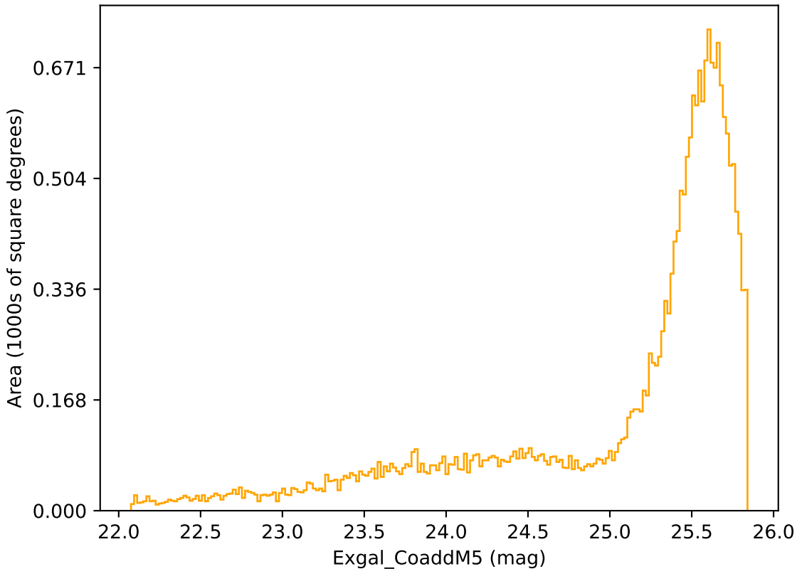
noroll_mjdp365_v3.4_10yrs Yr 3-4 r band: Exgal_CoaddM5
