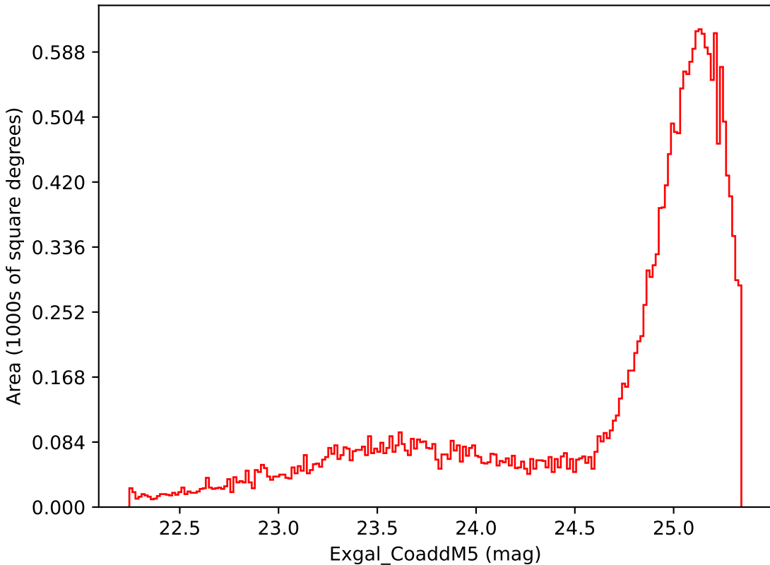
noroll_mjdp365_v3.4_10yrs Yr 3-4 i band: Exgal_CoaddM5
