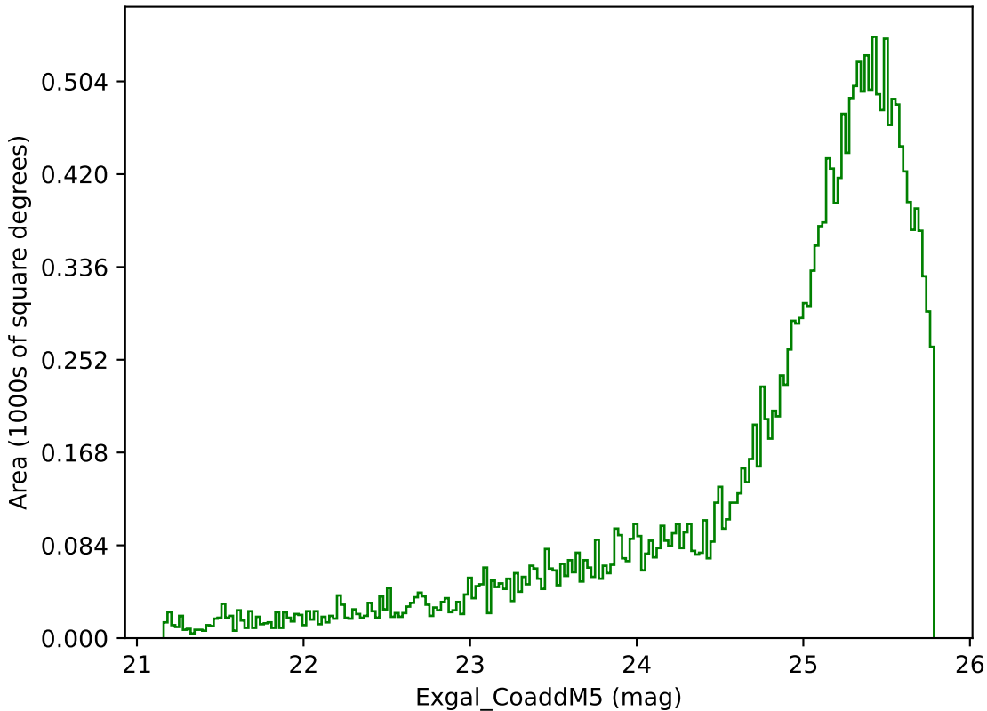
noroll_mjdp365_v3.4_10yrs Yr 3-4 g band: Exgal_CoaddM5
