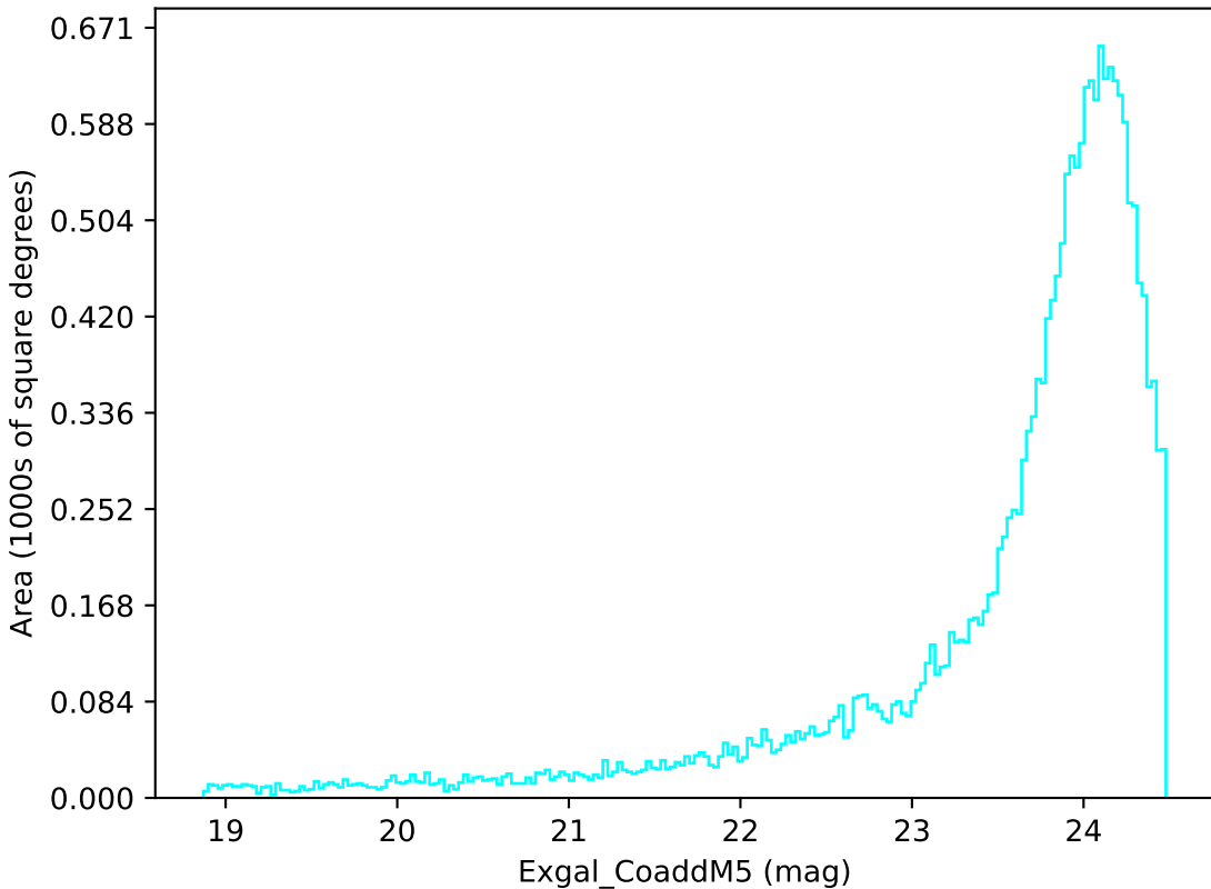
noroll_mjdp365_v3.4_10yrs Yr 1 u band: Exgal_CoaddM5
