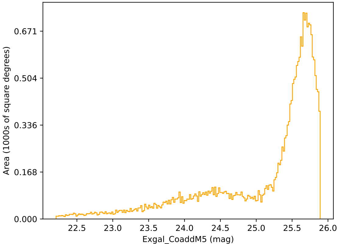
noroll_mjdp365_v3.4_10yrs Yr 1 r band: Exgal_CoaddM5
