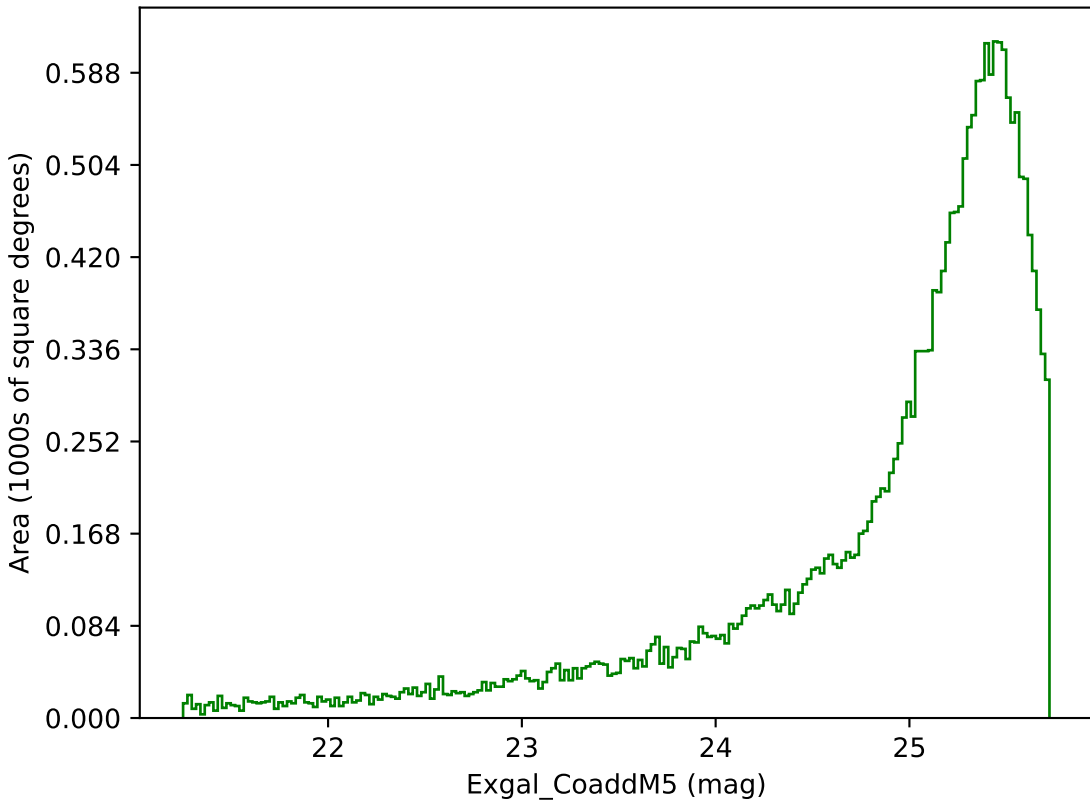
noroll_mjdp365_v3.4_10yrs Yr 1 g band: Exgal_CoaddM5
