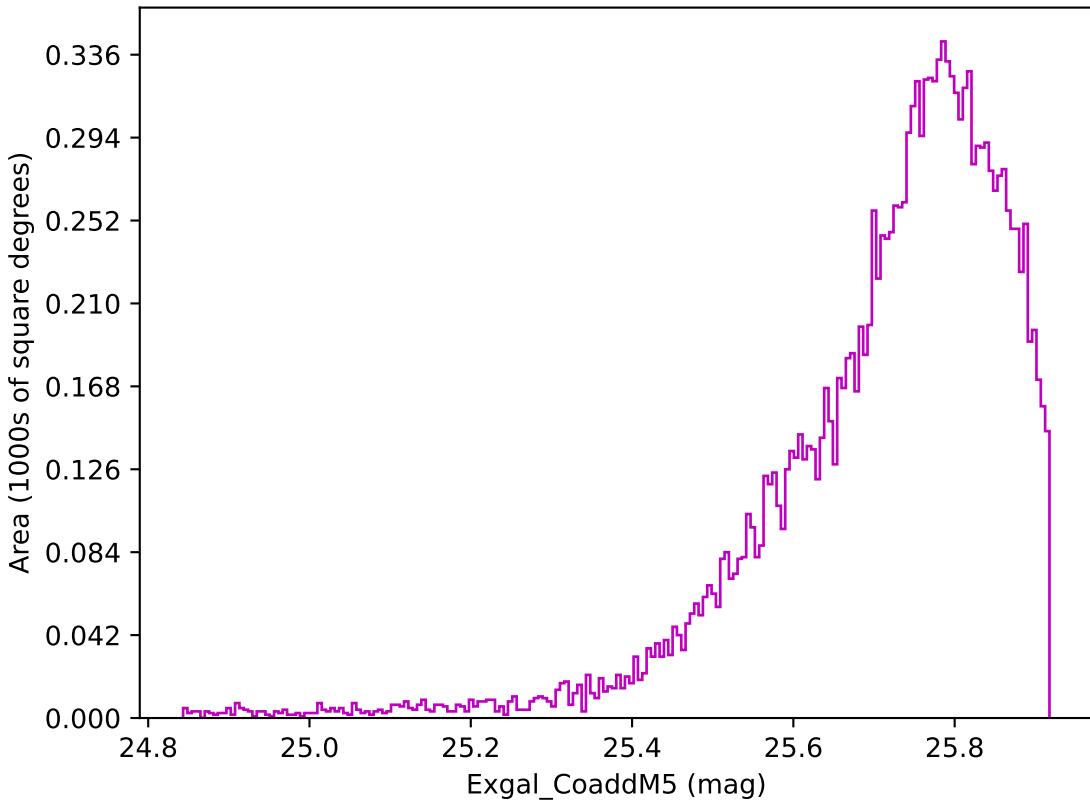
noroll_mjdp365_v3.4_10yrs WFD z band: Exgal_CoaddM5
