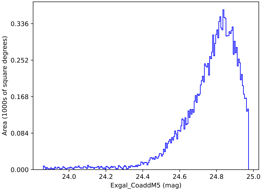
noroll_mjdp365_v3.4_10yrs WFD y band: Exgal_CoaddM5
