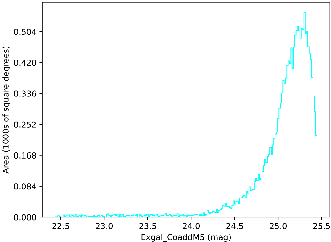
noroll_mjdp365_v3.4_10yrs WFD u band: Exgal_CoaddM5
