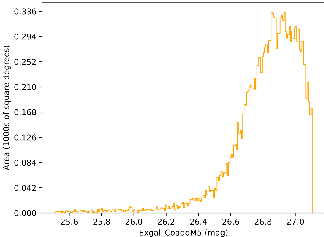
noroll_mjdp365_v3.4_10yrs WFD r band: Exgal_CoaddM5
