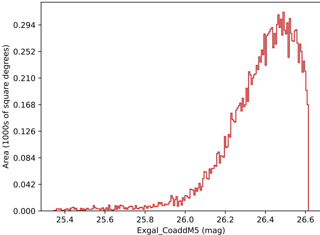
noroll_mjdp365_v3.4_10yrs WFD i band: Exgal_CoaddM5
