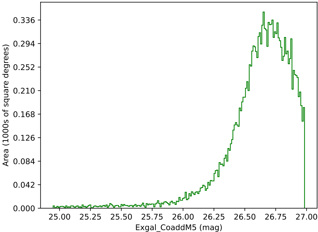
noroll_mjdp365_v3.4_10yrs WFD g band: Exgal_CoaddM5
