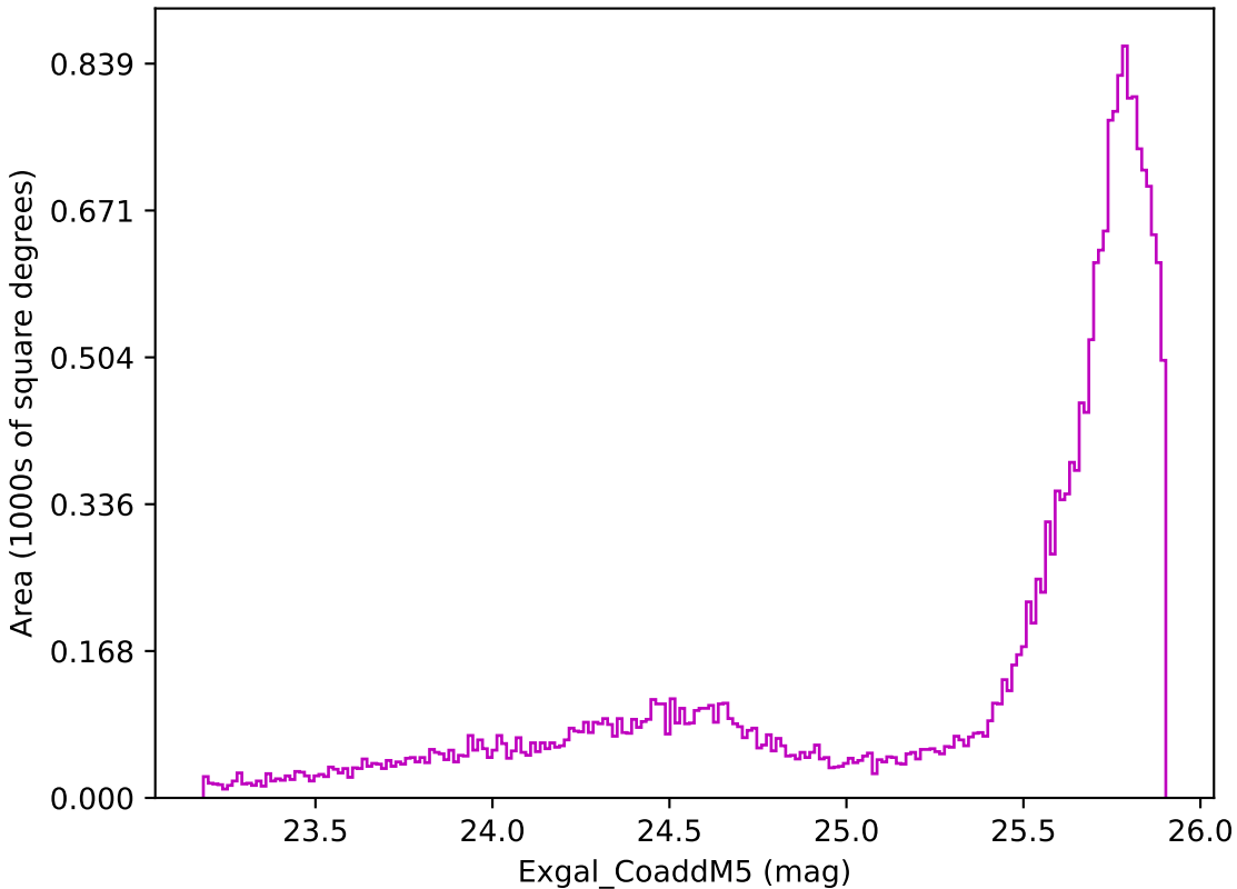
noroll_mjdp365_v3.4_10yrs All sky z band: Exgal_CoaddM5
